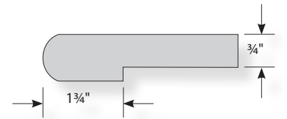
OAK RETURN NOSING
